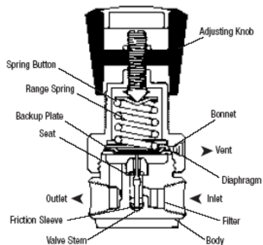
Figure 1 Single-stage regulator
